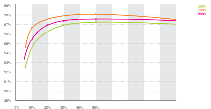
Growatt 40000 TL3 efficiency
